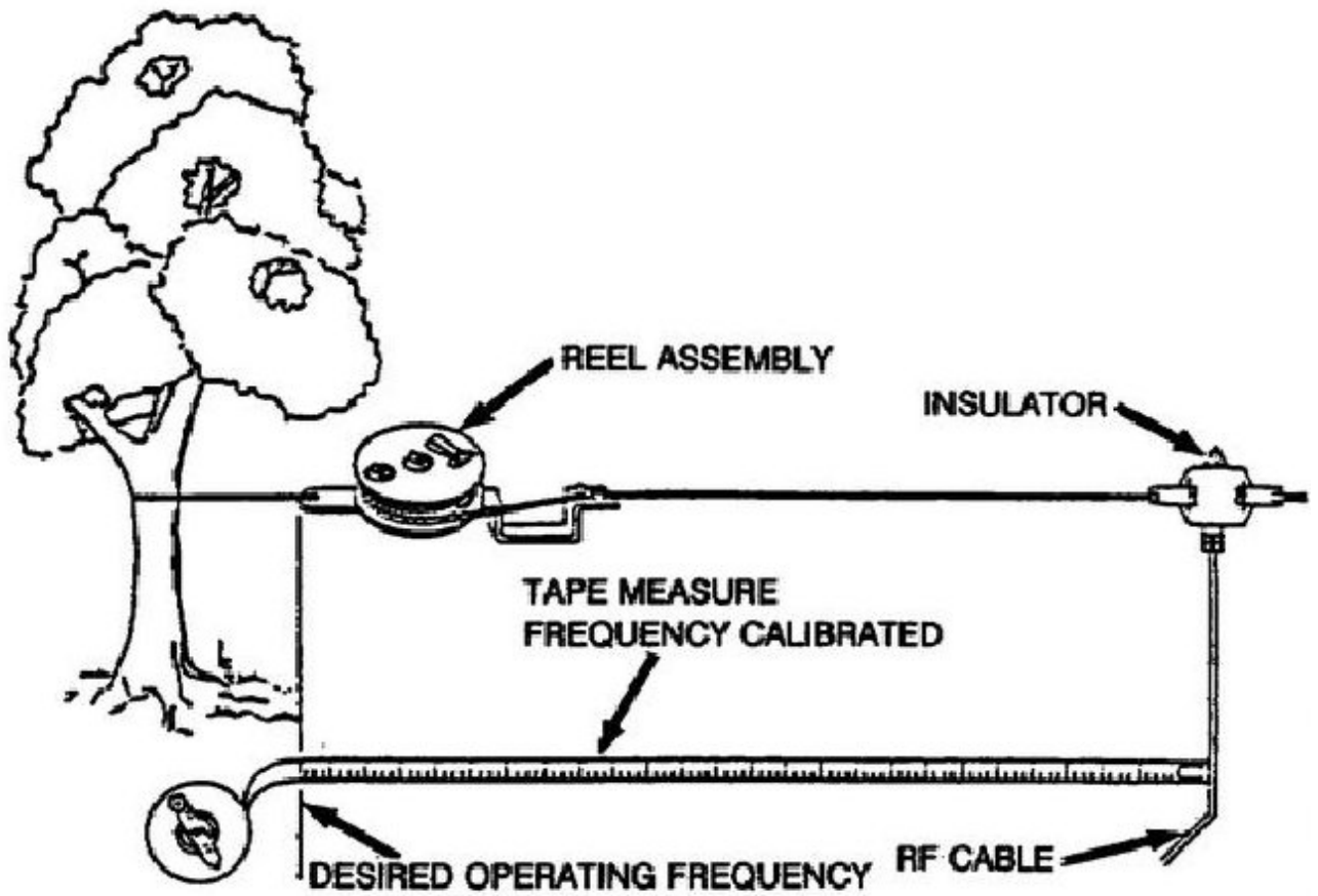
USE OF TAPE MEASURE TO DETERMINE ANTENNA WIRE LENGTH
