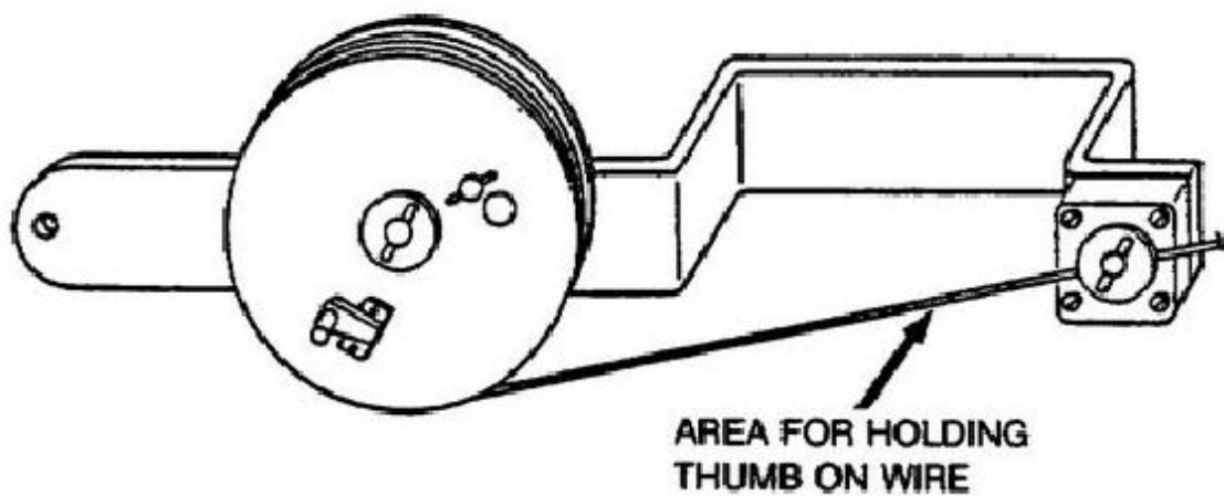
UNWINDING ANTENNA WIRE FROM REEL ASSEMBLY
